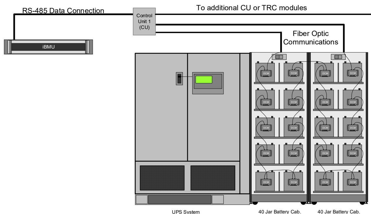
Figure 2, Control Unit and Partial System
