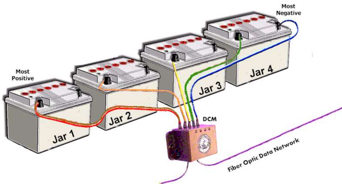
Figure 3, DCM connection.
