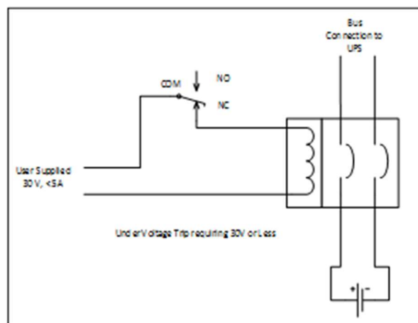
Example UV Trip using 30V or less
