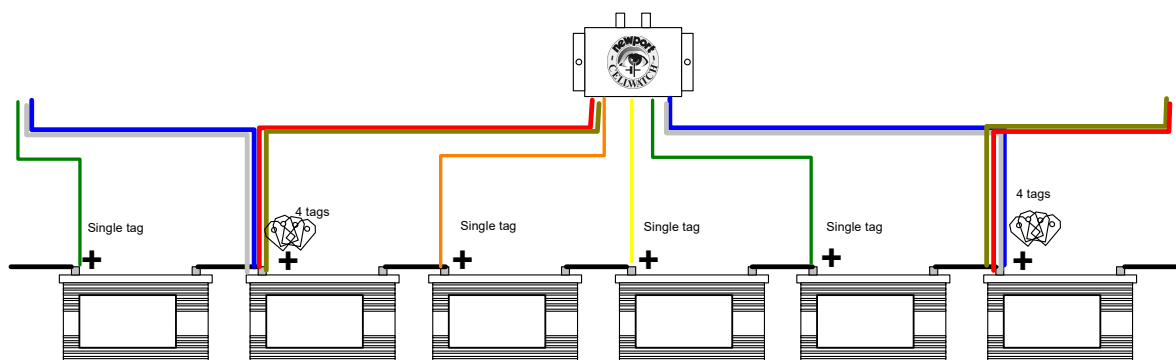
Battery Connection: Every Positive Post method.
