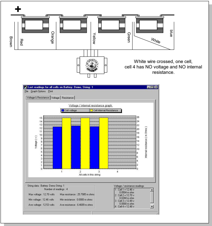
Crossed Wires show near zero readings for some cells
