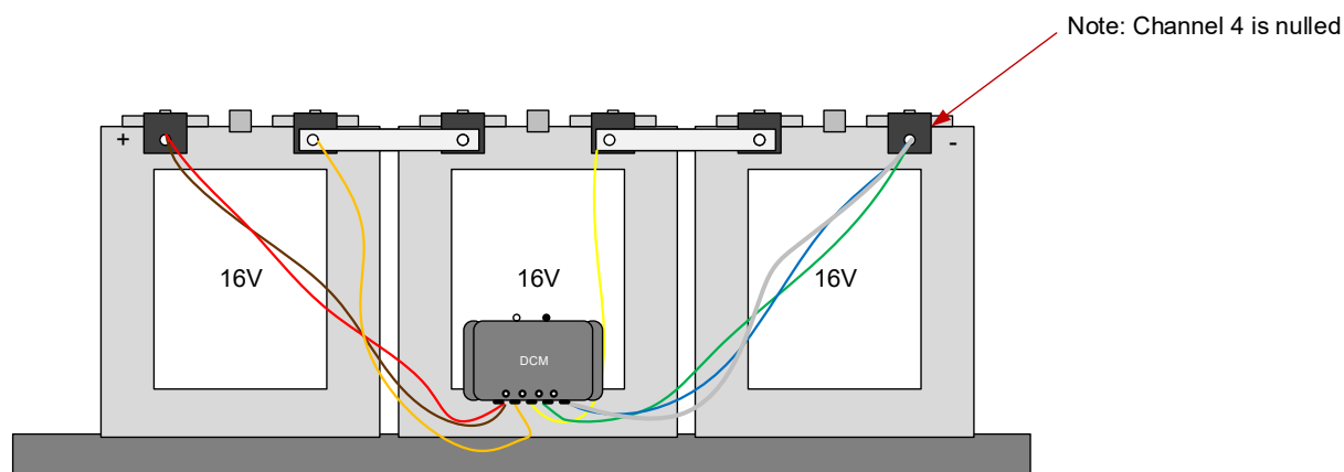
Figure 4 Short Tray Solution
